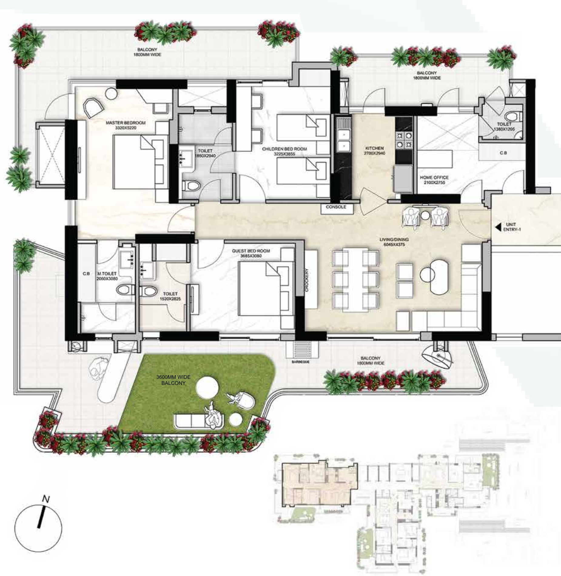
KEY PLAN: TWENTY FIRST FLOOR
